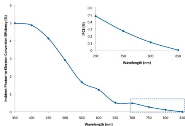
Figure 7. IPCE from a BAs crystal calculated from the net photocurrent (the overall current minus the dark current) at -0.25 V vs. Ag/AgCl in a 0.1 M aqueous Na 2 SO 4 solution containing 0.01 M methyl viologen. The inset shows the marked box on an expanded scale.
