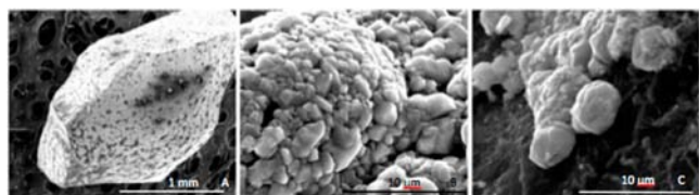
Figure 1. SEM images revealing the surface and core structure of the BA s -containing material prepared from granular boron. (A) A single piece of BA s . (B) Area of continuous BA s surface coverage. (C) Area featuring a gap in the surface coverage. The light material is BA s and the dark material is the boron substrate.
