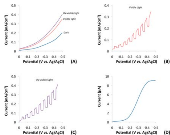
Figure 4. LSVs in a 0.1 M aqueous Na 2 SO 4 solution containing 0.01 M methyl viologen. The potential was swept from 0.0 to –0.5 V vs Ag/AgCl at a scan rate of 20 mV/s. The incident light intensity at the electrode surface was 100 mW/cm 2 . (A) Current flow for the new BA s material in the dark, under visible light and UV–vis irradiation. (B) Current flow for the BA s material under chopped visible light irradiation. (C) Current flow for the BA s material under chopped UV–vis irradiation. (D) LSV of an As-doped boron electrode in the dark.
